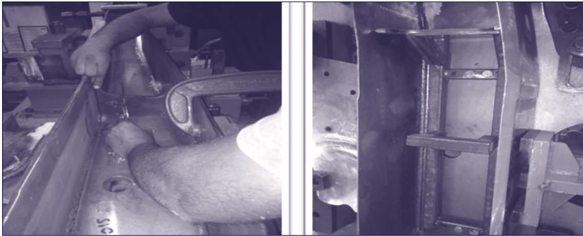
Template for Diaphragm Set up at Side Frame Set Up – Stage Fig. 6 Modification in diaphragm set-up (Before and after condition)
